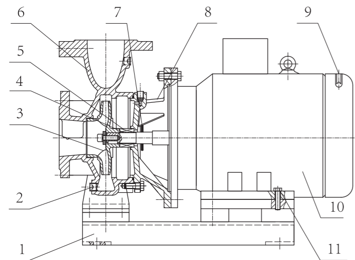
KQW结构图 KQW STRUCTURE DRAWING
