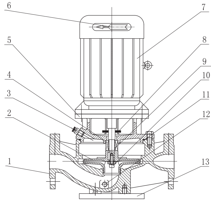
KQW结构图 KQW STRUCTURE DRAWING
